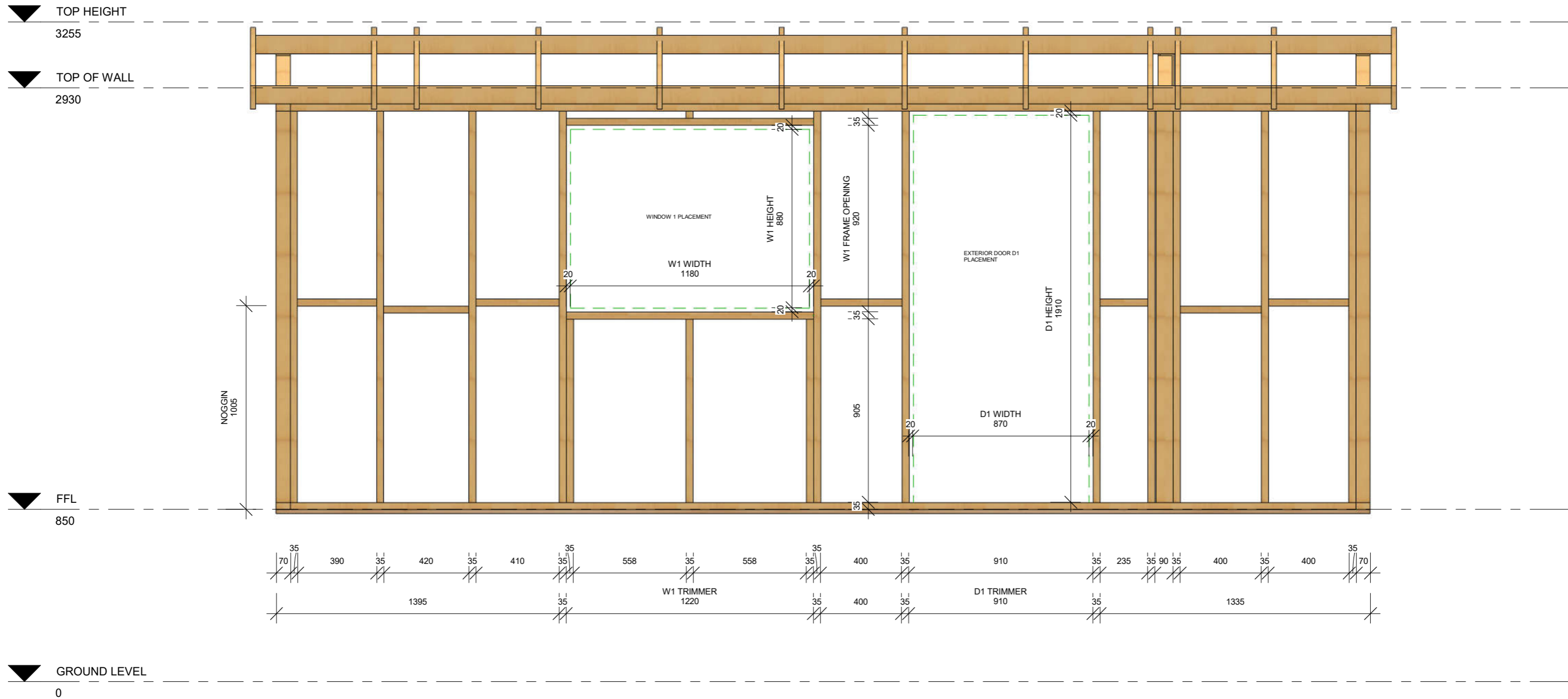
1 NORTH WALL FRAME 1 : 20
