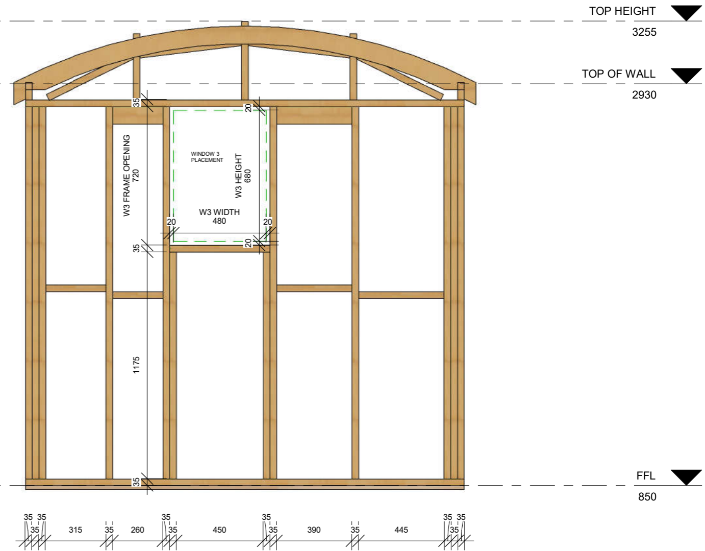
4 WEST WALL FRAME 1 : 20
