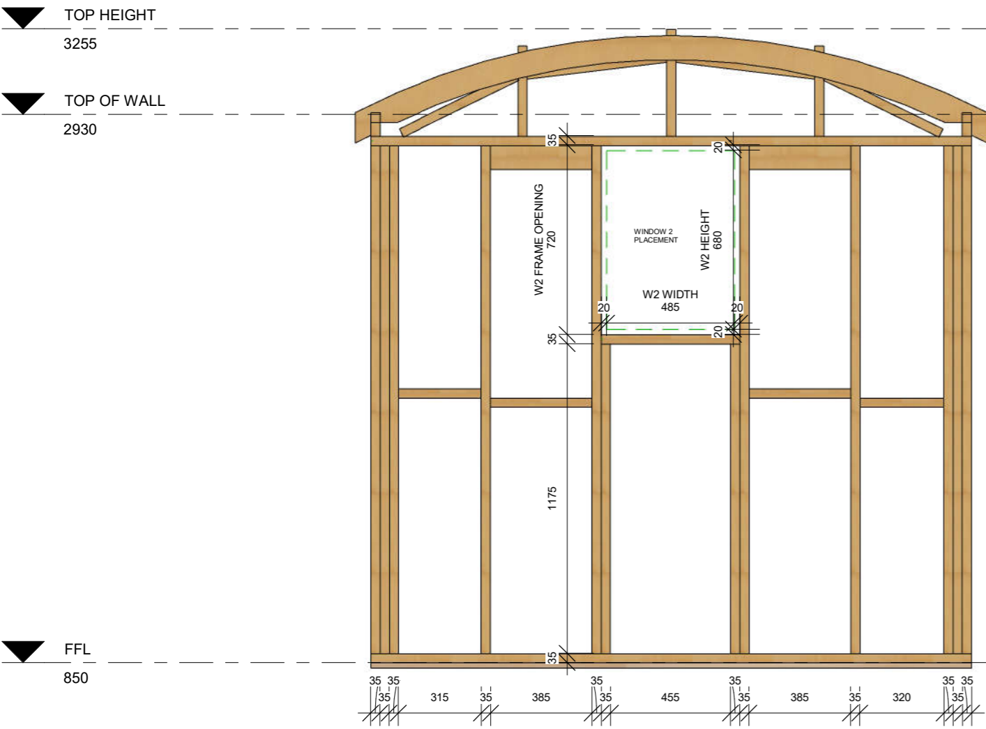
3 EAST WALL FRAME 1 : 20
